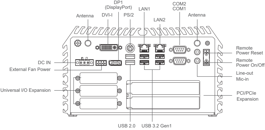
Rear I/O
