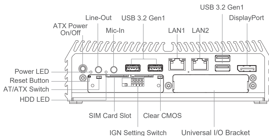
Front I/O
