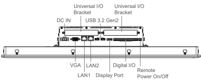
Rear I/O
