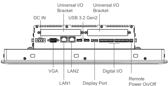
Rear I/O
