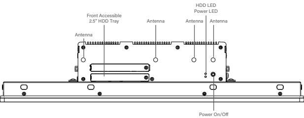
Front I/O
