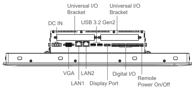
Rear I/O
