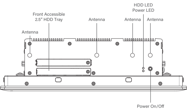
Front I/O
