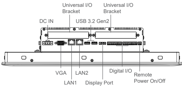
Rear I/O
