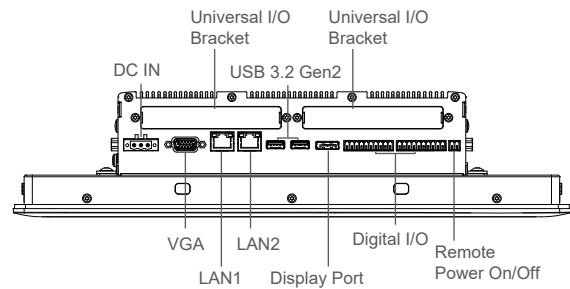
Rear I/O
