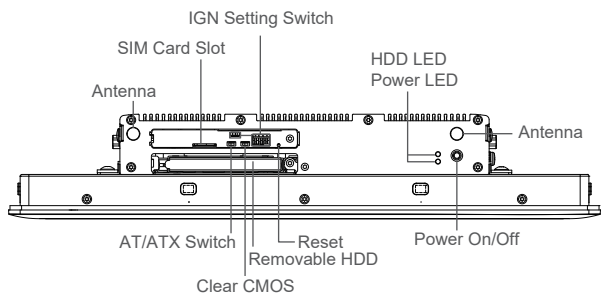
Front I/O
