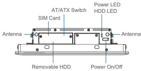
Front I/O
