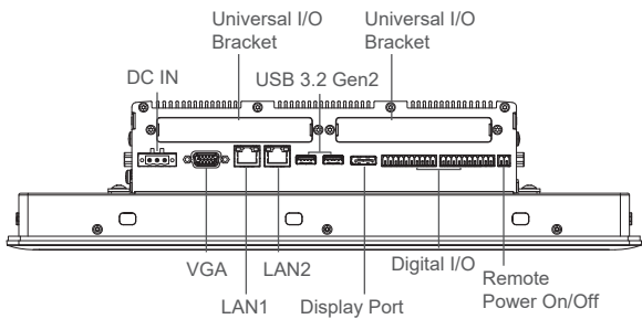
Rear I/O
