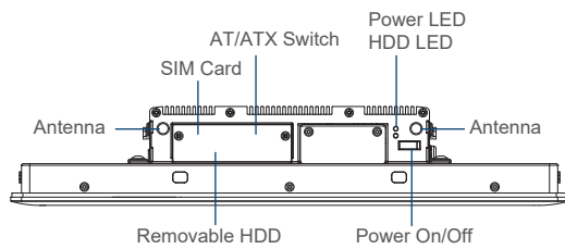
Front I/O
